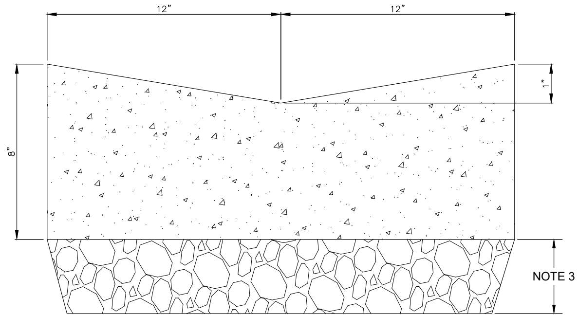
VALLEY GUTTER
