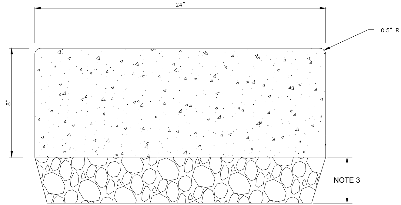
FLAT CURB
